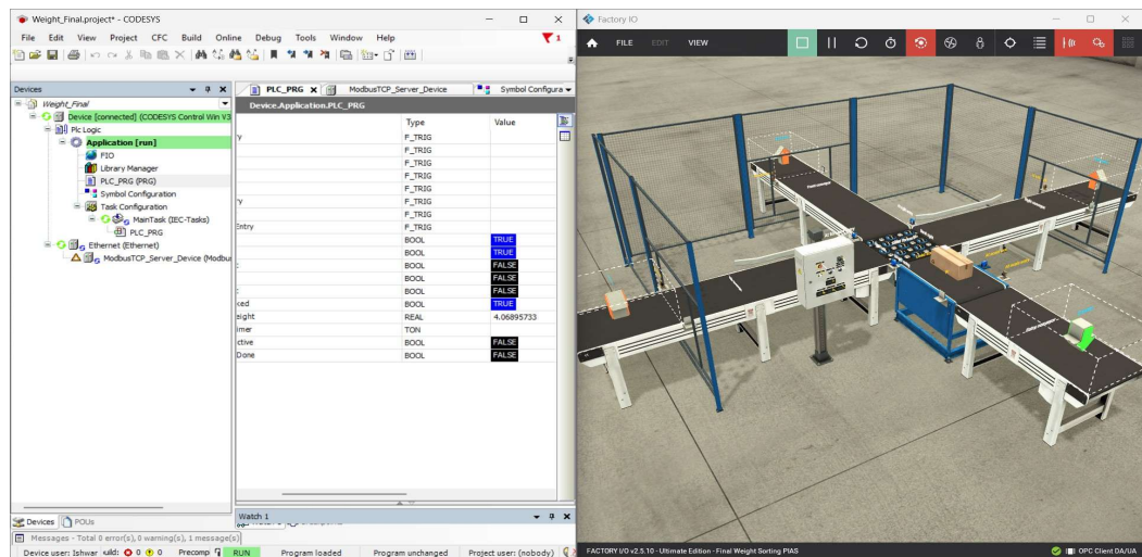
Fig 5.2 System Integration working with Real-Time data exchanging through OPC UA protocol with side-by-side clear visualization.
