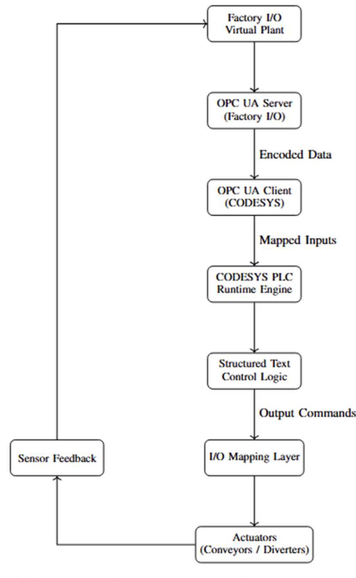
Fig. 6. Communication protocol diagram showing the complete OPC UA data flow between Factory I/O, OPC UA server/client layers, and CODESYS PLC control logic.
