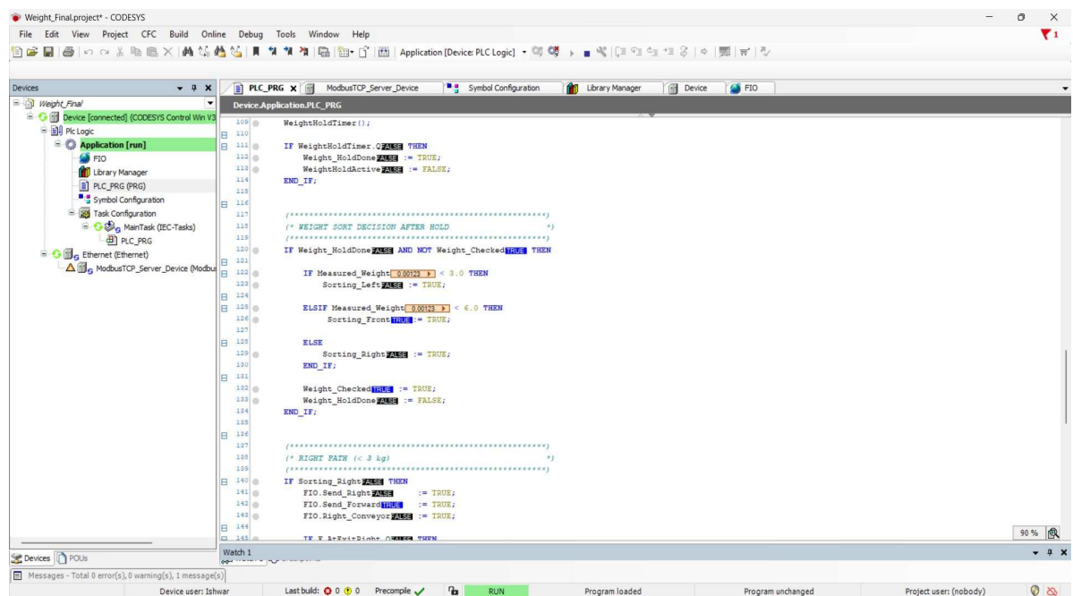
Fig 5.1 Through OPC UA Communication protocol, how the instruction set is running with Real-Time data exchanging between Factory IO and CODESYS.
