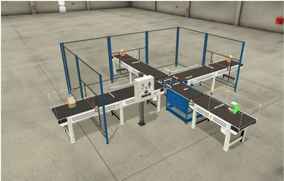
Fig 4.3: Factory IO Sensors and Actuators virtual assembly in Factory IO.
